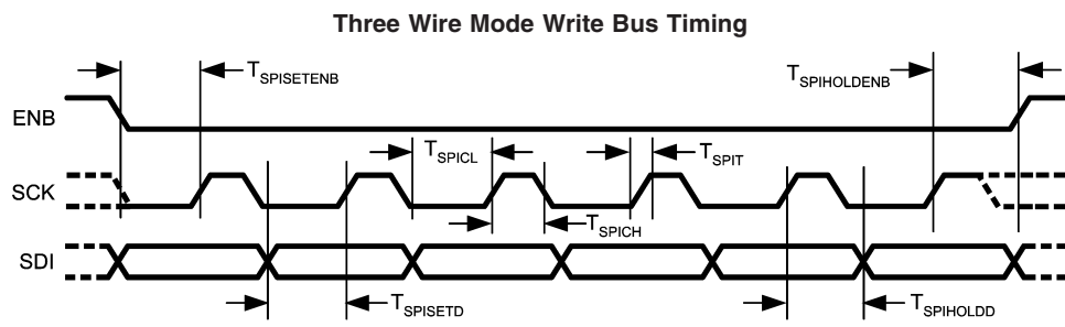
FIGURE 3. Three Wire Mode Write Bus
